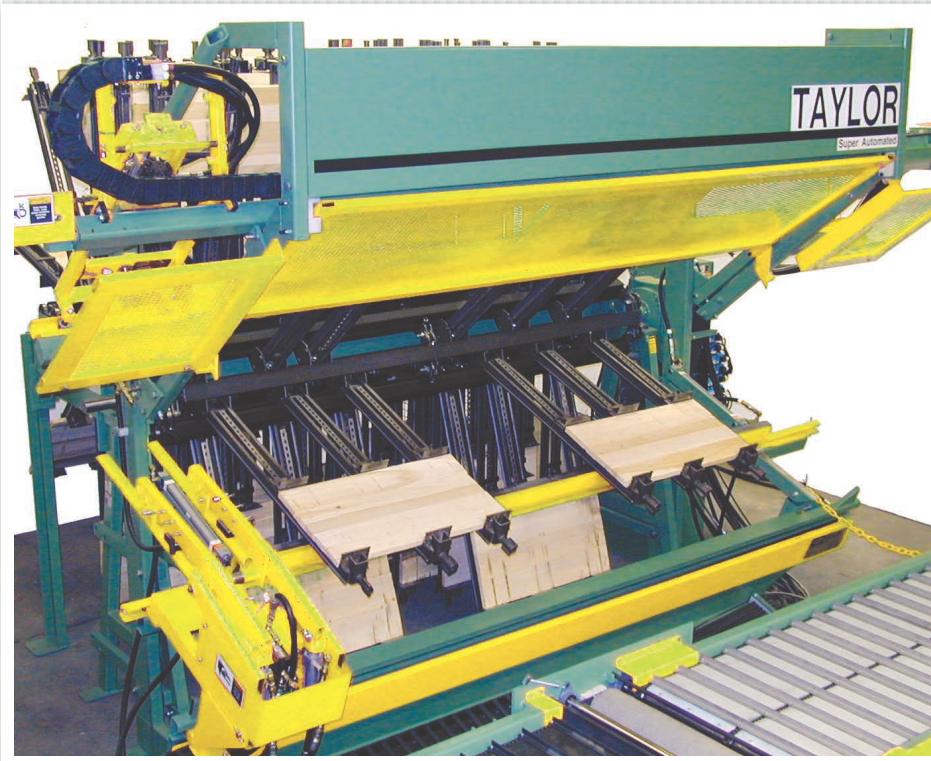
8 1/2' 40 section Super Automated Clamp Carrier
