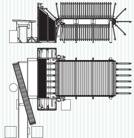
8-1/2' Wide, 60 Section Dual Automated Clamp Carrier with Glue Applicator & Return Conveyor.
